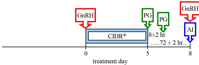
Figure 4. Beef cow fixed-time AI protocols.*
