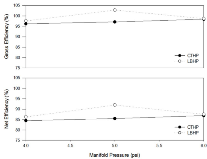
Figure 2. Effect of varying manifold pressure on gross and net combustion efficiency of high-pressure radiant brooders. The middle point in each line graph represents the rated manifold pressure for the respective brooder.
