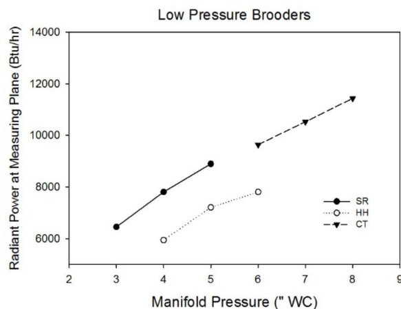
Figure 4. Effect of varying manifold pressure on total radiant power at the measuring plane of low- and high-pressure round radiant brooders. The middle point in each line graph represents the rated manifold pressure for the respective brooder.
