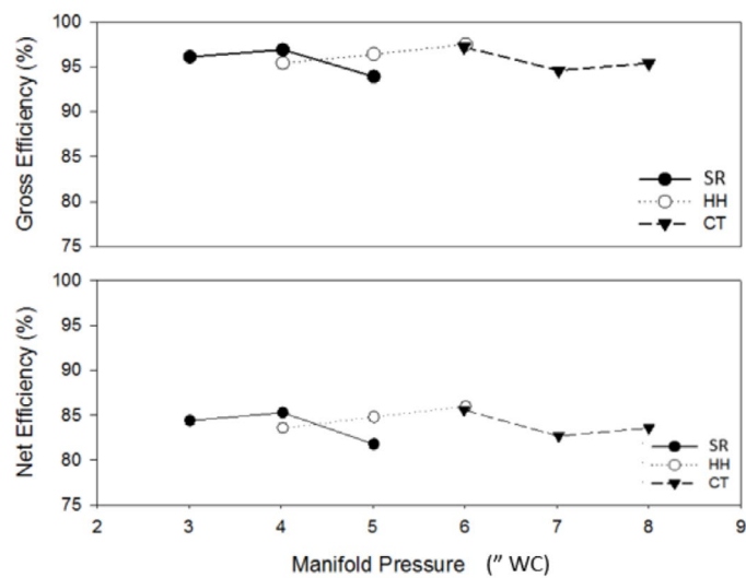
Figure 1. Effect of varying manifold pressure on gross and net combustion efficiency of low-pressure radiant brooders. The central point in each line graph represents the rated manifold pressure for the respective brooder.
