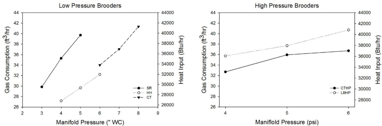
Figure 3. Effect of varying manifold pressure on gas consumption and heat input of low- and high-pressure round radiant brooders. The middle point in each line graph represents the rated manifold pressure for the respective brooder.
