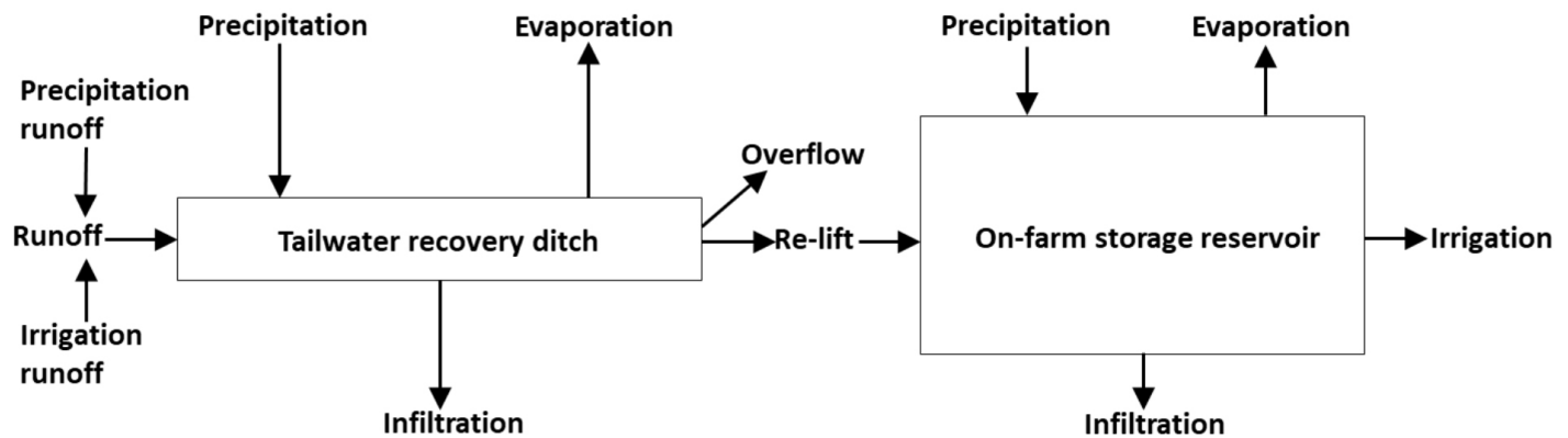
Figure 3. Gains and losses of water into and out of TWR systems. Figure from Omer et al. (2017).
