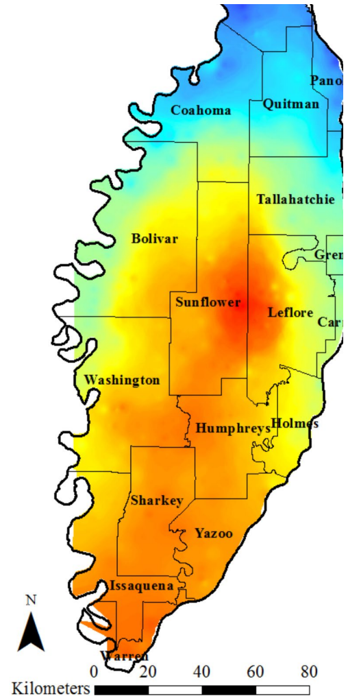
Figure 1. Ground water levels in the Mississippi Delta. Groundwater data were provided by Yazoo Mississippi Delta Joint Water Management District.
